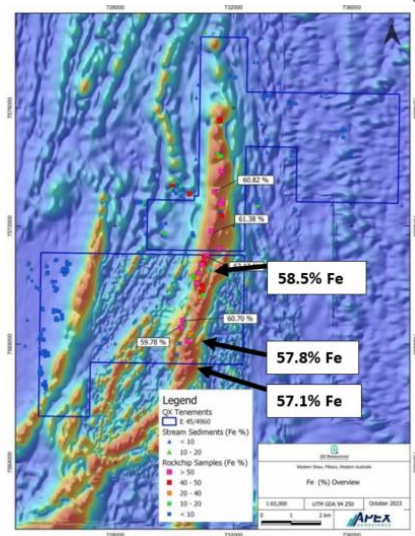
Figure 2: Best rockchip iron ore assays (Fe%) – QXR samples (Large Text) and Historical Atlas Iron samples (small text) + located on a magnetic image over Western Shaw, Pilbara
