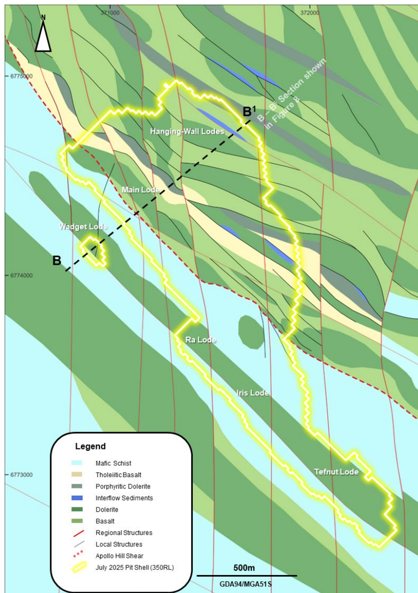
Figure 7 – Apollo Hill Geological Interpretation (also see cross section B-B' in Figure 8).
