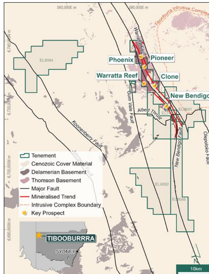
Figure 4: Geology and main prospects of the Tibooburra tenements highlighting the Albert Goldfields at the boundary of the Thomson and Delamerian orogens wrapping around the west side of a cluster of large granite intrusions to the east.
