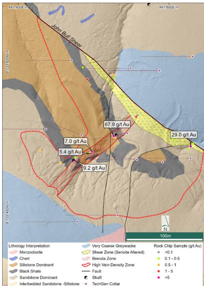
Figure 3 John Bull Main Workings interpreted geology showing preferred stratigraphy and high vein density areas, with rock chip results where outcrop can be identified. 2
