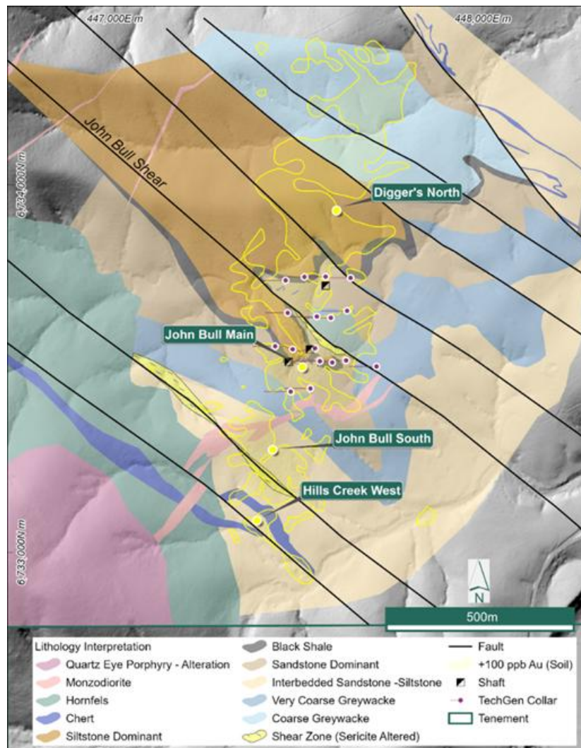
Figure 2 Regional geological interpretation map of the John Bull Project over LiDAR™ showing Key Target Area locations.
