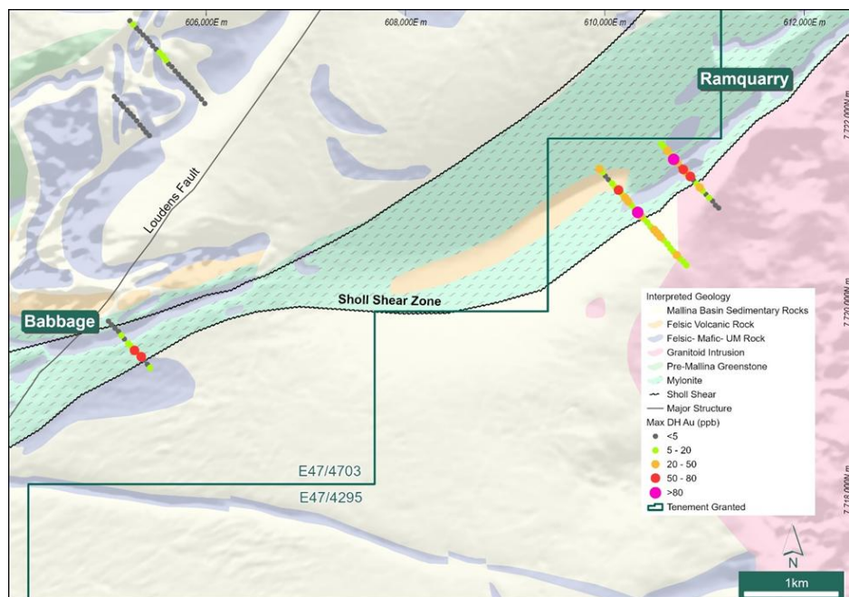
Figure 10: AC collar locations over regional geological interpretation and airborne magnetics, showing maximum downhole gold values.
