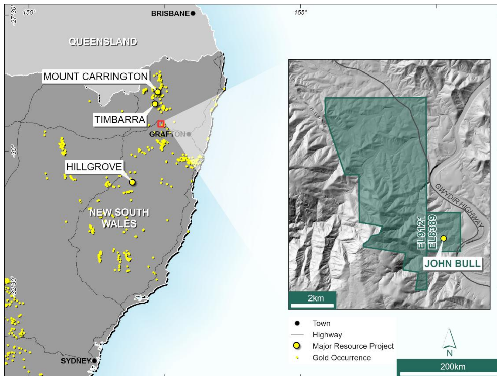
Figure 1: Location of the John Bull Gold Project in northeastern NSW, Australia.
