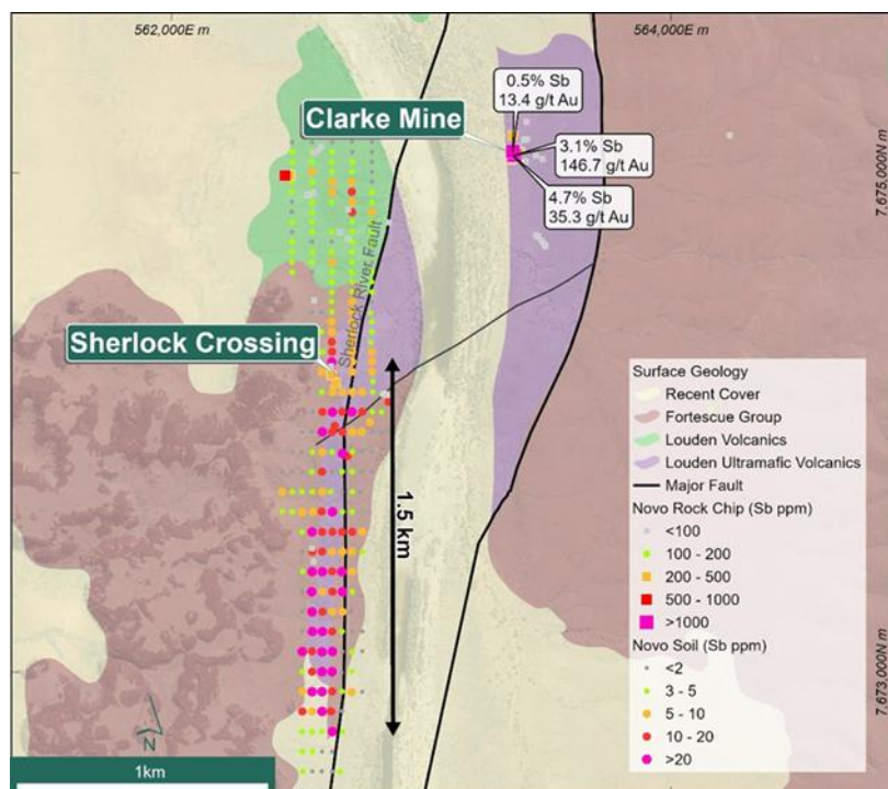
Figure 11: Sherlock Crossing, showing extended soil anomaly > 15 ppm Sb to the SW of the proposed first pass drilling area at the Clarke Mine 5
