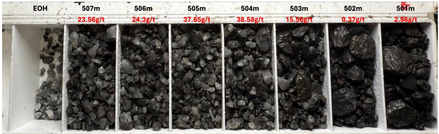
Figure 3 RC drill chips, abundant pyrrhotite, sulphides and vein quartz representing 7m @ 20.43 g/t gold , including 5m @ 27.93 g/t gold .
