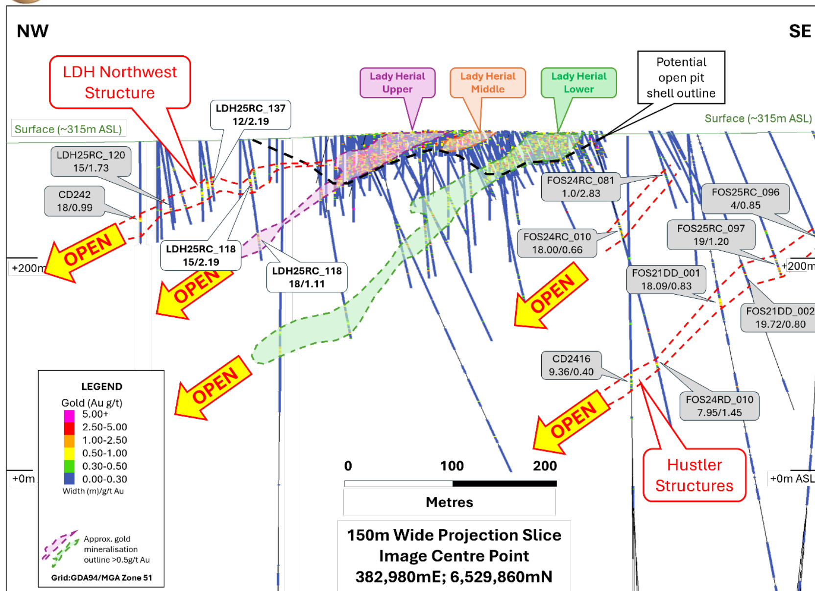
Figure 3: Long sectional projection view, looking towards the northeast, illustrating the proximity and relationship between LDH Northwest, annotated with select new drill intercepts (white call-outs), and the Lady Herial and Hustler structures with previously reported drill intercepts (grey call-outs, see ASX announcements dated 10 Oct and 13 Dec 2024, and 18 Mar and 30 May 2025).
